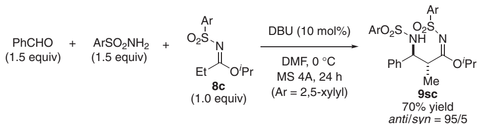
Scheme 3. 3-component reaction.
