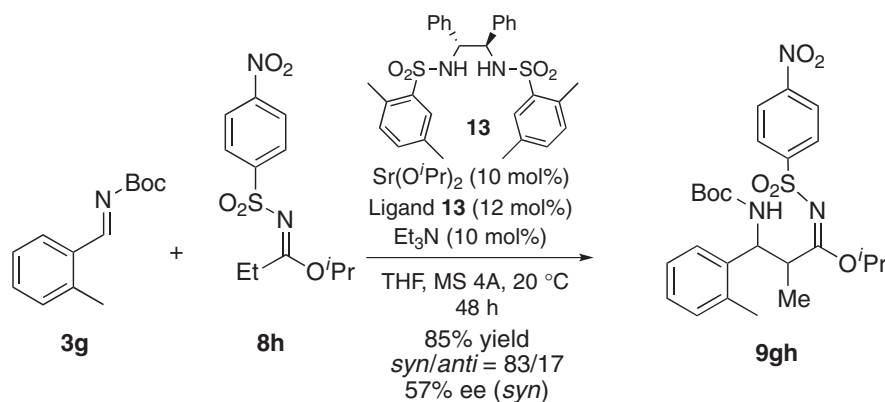
Scheme 5. Catalytic asymmetric addition reaction of sulfonylimide with N -Boc imine.
