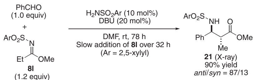
Scheme 10. Direct formation of \beta -amino acid ester from aldehyde and sulfonylimide.
