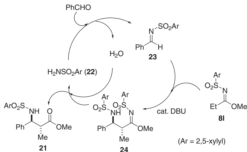
Figure 9. Formation of \beta -amino acid ester.
