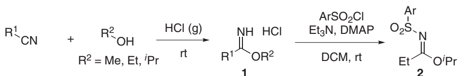
Scheme 1. Synthetic method of sulfonylimidate.
