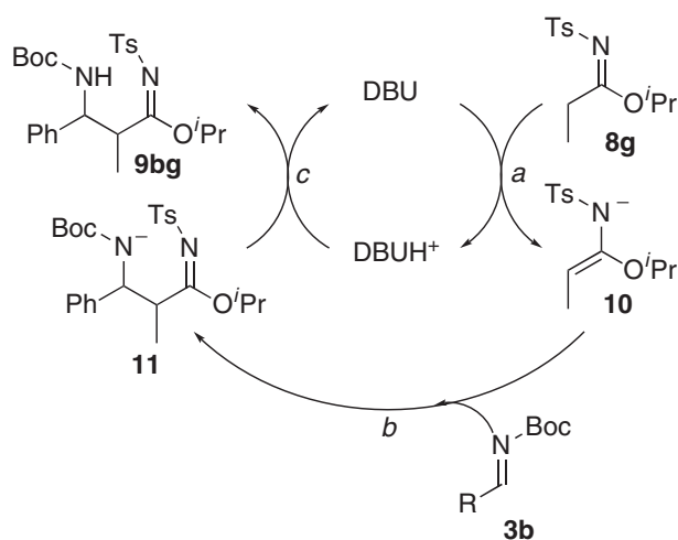
Figure 4. Catalytic cycle.
