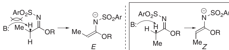
Scheme 6. Proposed geometry of aza-enolate derived from sulfonylimide.
