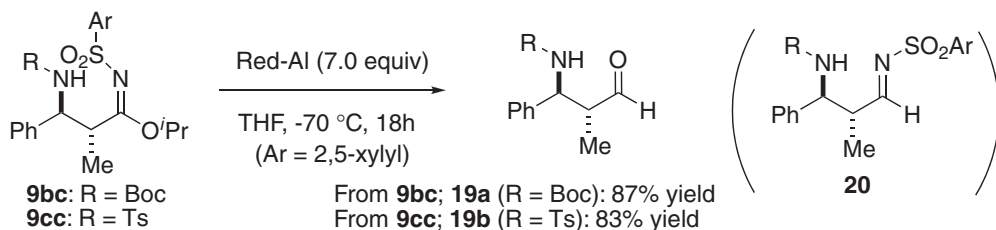
Scheme 9. Conversion of the products (3).
