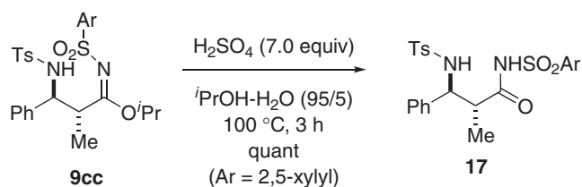
Scheme 7. Conversion of the products (1).
