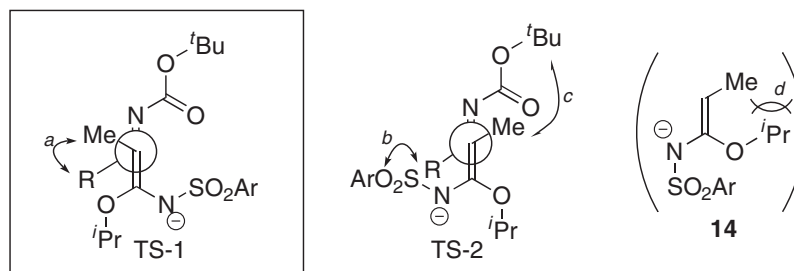
Figure 6. Proposed transition state model.
