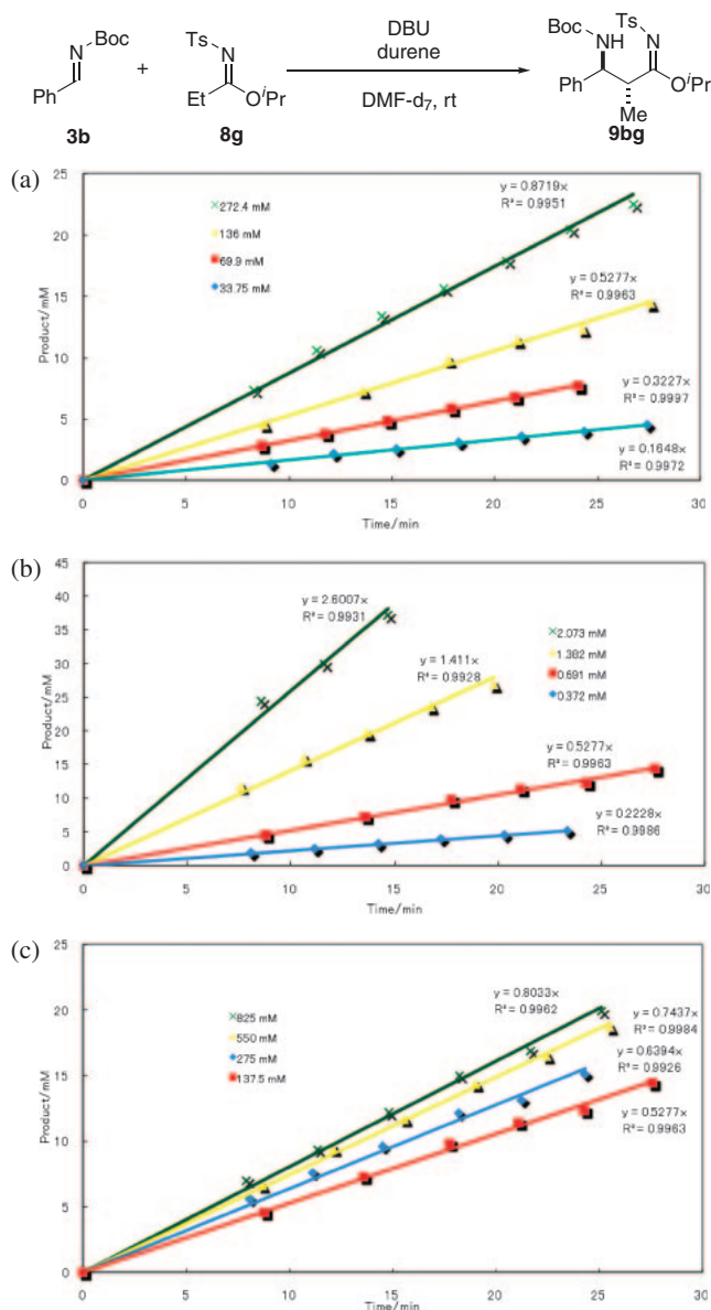
Figure 2. Initial reaction profile varying the concentration of (a) sulfonylimide 8g , (b) DBU, and (c) Boc imine 3b .
