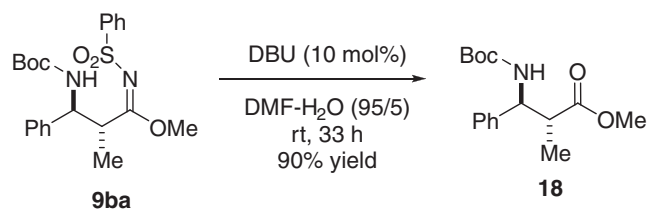
Scheme 8. Conversion of the products (2).
