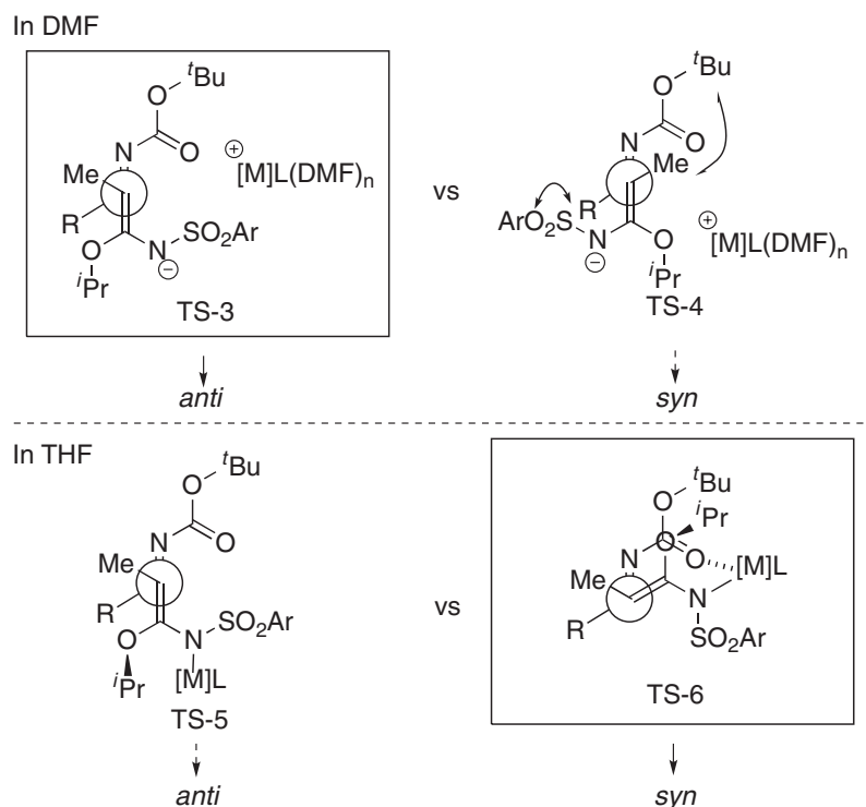
Figure 7. Proposed transition state models (L = ligand).
