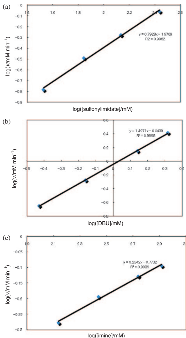
Figure 3. Determination of reaction dependence on (a) sulfonylimide 8g , (b) DBU, and (c) Boc imine 3b .
