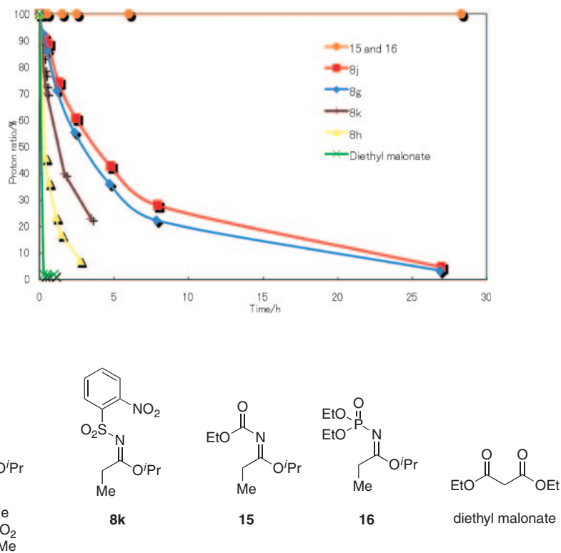
Figure 8. Deuterium exchange experiment of active methylene compounds.
