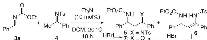
Scheme 2. Direct-type reaction of sulfonylimine 4 with imine 3a .
