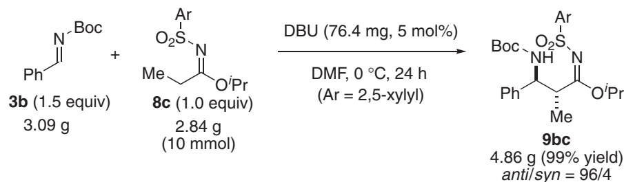
Scheme 4. Large scale synthesis.
