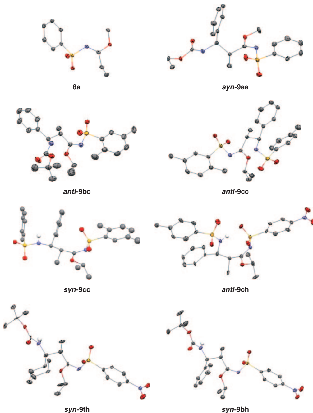
Figure 5. X-ray crystal structures of the products.
