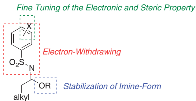
Figure 1. Sulfonylimide as a nucleophile.
